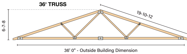
STANDARD STOCK TRUSS
